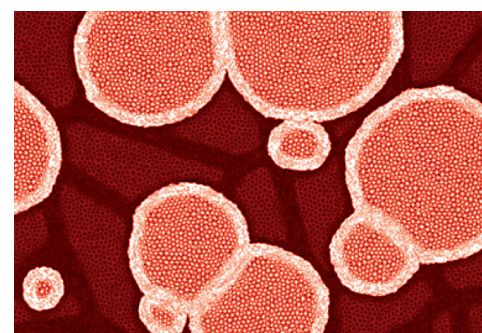
2D simulation of primary recrystallization with an initial uniform stored energy M Bernacki, H Resk, T Coupez and R E Logé 2009 Modelling Simul. Mater. Sci. Eng. 17 064006.
